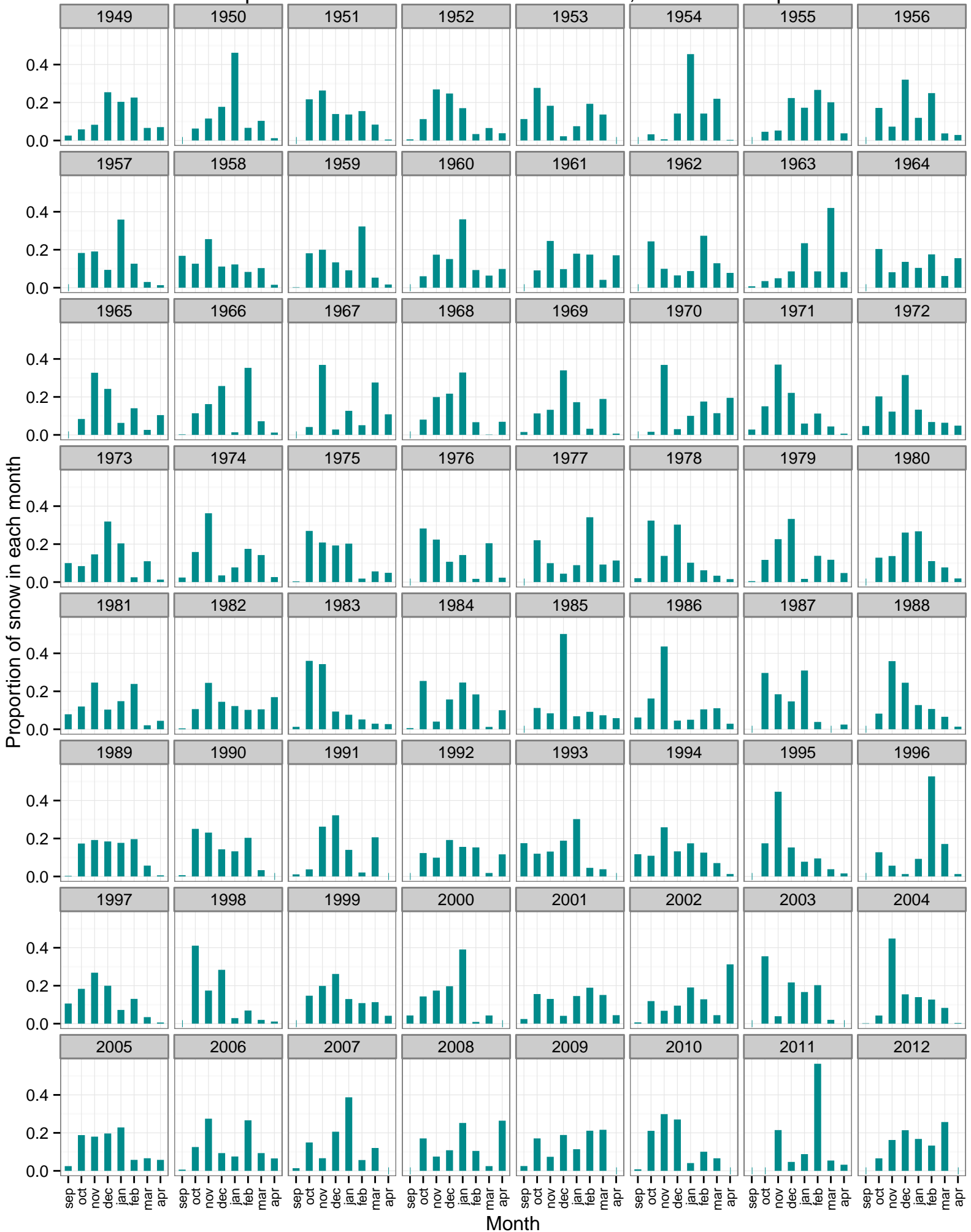
Proportion of total snowfall in each month, Fairbanks Airport
