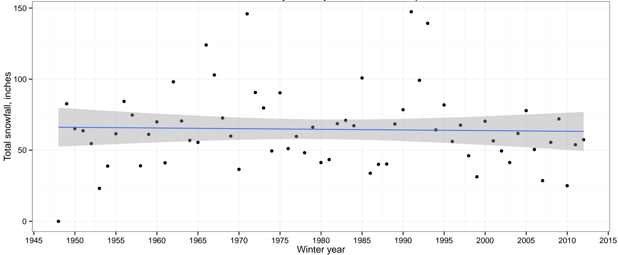
Total snowfall by winter year, Fairbanks Airport
