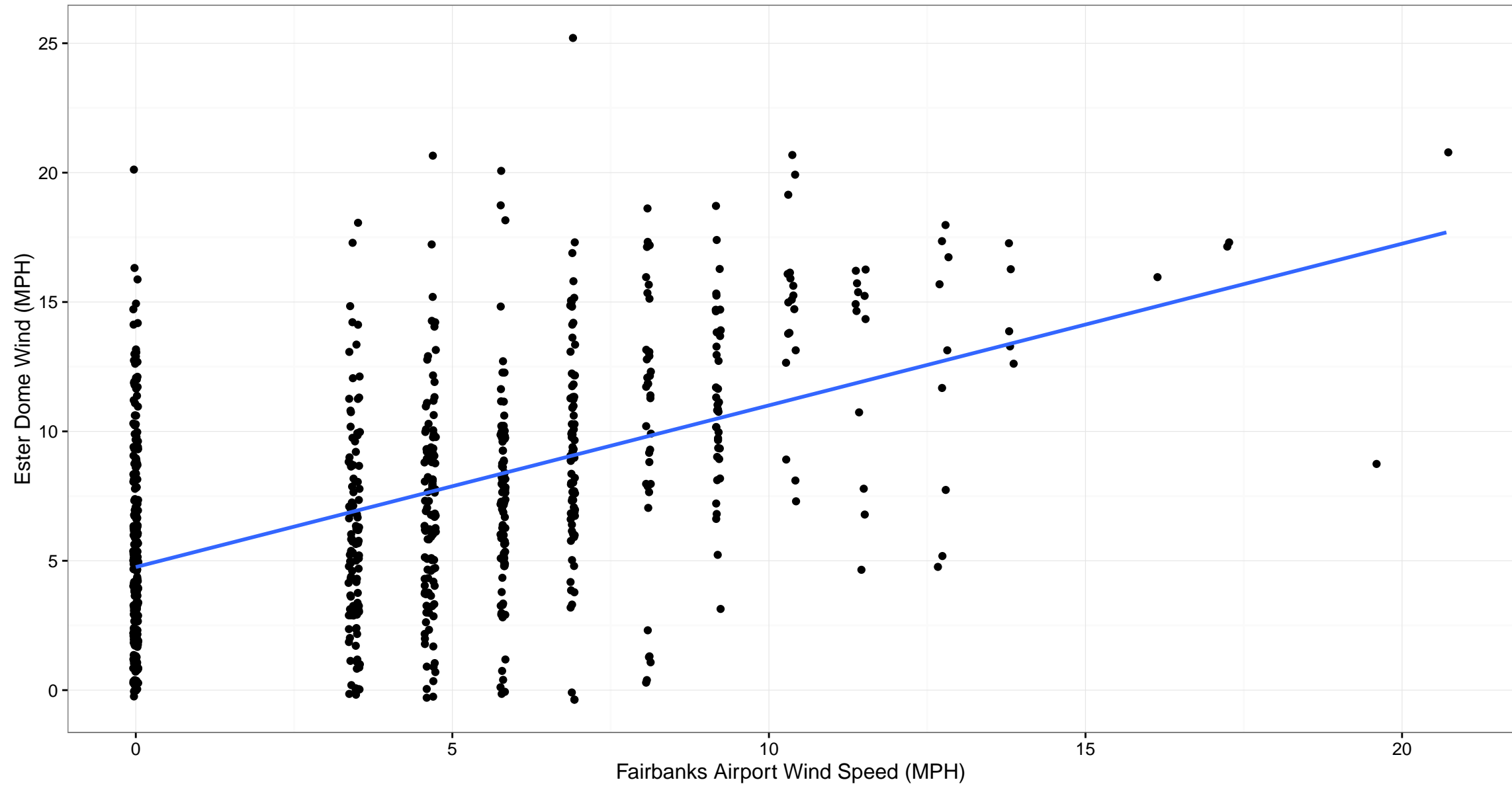
Relationship between Fairbanks Airport and Ester Dome Wind Speeds September, 2008–2013
